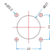
安装开孔图 Installation hole figure
