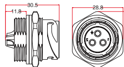
插座 SX (外型尺寸图) SX socket (dimensions figure)
