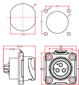
安装开孔图 Installation hole figure
